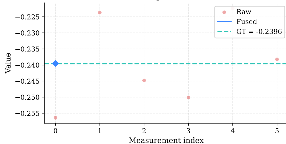
Component: z
