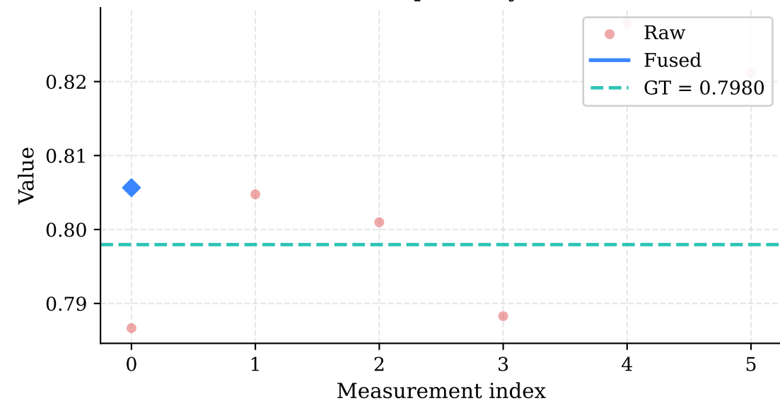
Component: w
