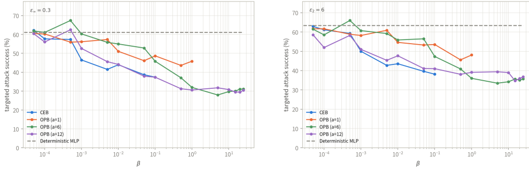
Figure 3: Targeted white-box PGD on MNIST (MLP). Left: L_\infty , \epsilon = 0.3 ; right: L_2 , \epsilon = 6 . Curves use the stochastic path and are shown only where clean accuracy exceeds 90%. Transfer curves are in Appendix B.5.
