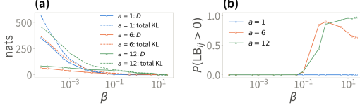
Figure 1: Alignment and separation diagnostics over the ImageNet-100 compression sweep. (a) Anchor mismatch \hat{D} (solid) and total KL (dashed) against \beta , by anchor scale. (b) Fraction of class pairs with a positive separation lower bound.
