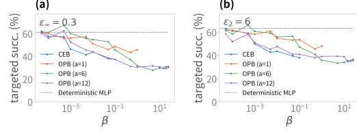
Figure 2: Targeted white-box PGD on MNIST (MLP): targeted success rate against \beta under (a) L_\infty , \epsilon = 0.3 and (b) L_2 , \epsilon = 6 . Curves are shown only where stochastic clean accuracy exceeds 90%.
