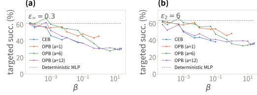
Figure 3: Targeted white-box PGD on MNIST (MLP). (a) L_\infty , \epsilon = 0.3 ; (b) L_2 , \epsilon = 6 . Curves use the stochastic path and are shown only where clean accuracy exceeds 90%. Transfer curves are in Appendix B.5.
