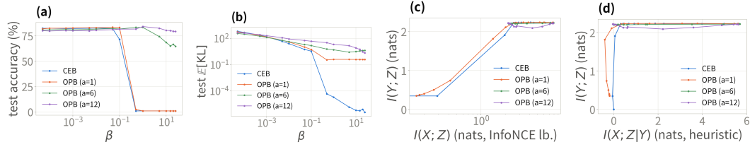
Figure 4: Compression diagnostics across two views and two tasks. (a)–(b) ImageNet-100 classification sweep (MLP): test accuracy and realized conditional KL against \beta ; CEB and the smallest anchor collapse at strong compression, whereas a = 12 retains the plateau. The Housing regression counterpart is provided in Appendix B.3. (c)–(d) MNIST information-plane and certificate-plane estimates (estimator-level diagnostics rather than mutual-information identities; Appendix B.4).
