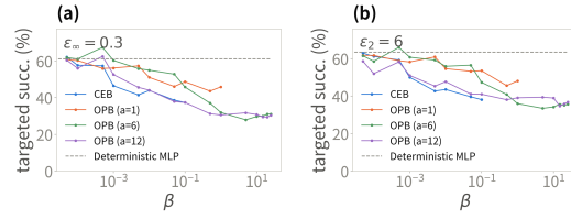
Figure 2: Targeted white-box PGD on MNIST (MLP). (a) L_\infty, \epsilon = 0.3 ; (b) L_2, \epsilon = 6 . Curves use the stochastic path and are shown only where clean accuracy exceeds 90%. Transfer curves are in Appendix B.5.
