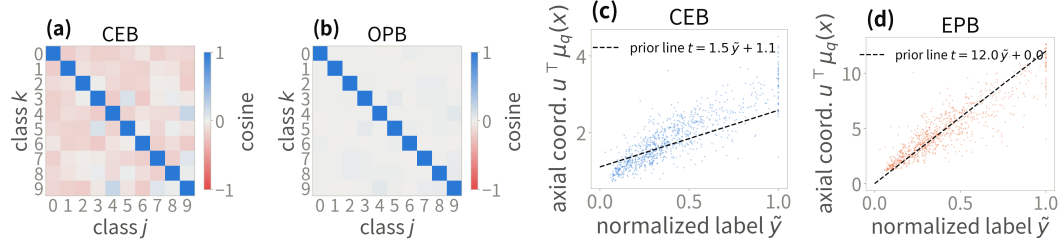
Figure 4: Posterior geometry: class-center Gram matrices for (a) CEB and (b) OPB, and axial coordinates for (c) CEB and (d) EPB.
