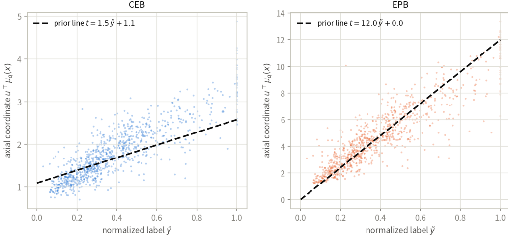
Figure 6: The axial coordinate u^\top \mu_q(x) against the normalized label on Housing (one representative run per model). The EPB posterior hugs the prior line \rho \tilde{y} , shrunk toward \rho \mathbb{E}[\tilde{y} | x] by the encoder’s uncertainty.
