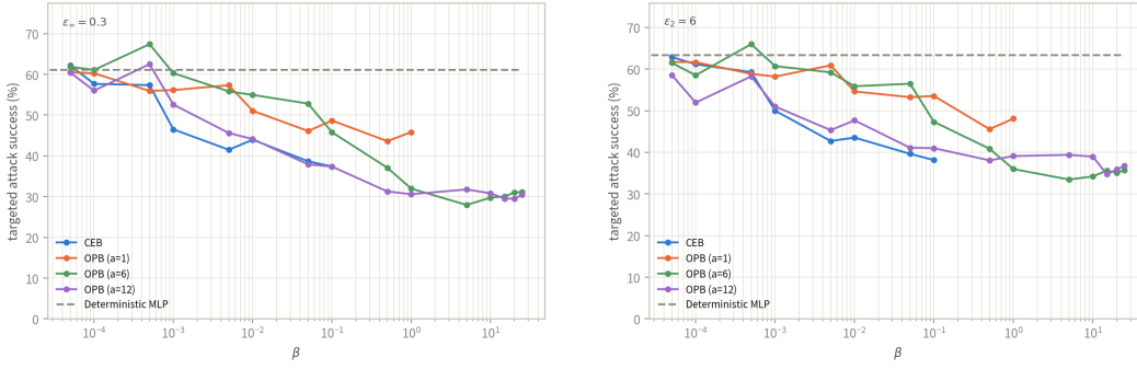
Figure 3: Targeted PGD attack success rate against \beta (log scale) on MNIST (MLP backbone): target class 0, 20 steps, EOT-10 gradients and 10-sample MC predictions on the stochastic path. (a) L_\infty , \varepsilon_\infty = 0.3 ; (b) L_2 , \varepsilon_2 = 6.0 . The dashed grey line is the deterministic MLP baseline. Every curve is drawn only over \beta values with clean accuracy above the shared 90% failure threshold (CEB: \beta \leq 0.1 ; OPB a = 1 : \beta \leq 1 ; a = 6, 12 : full grid). Every curve falls with \beta , and OPB keeps gaining robustness across its valid range: at \beta = 25 , OPB ( a = 6, 12 ) reach 31.1%/30.5% — about 30 points below the baseline.
