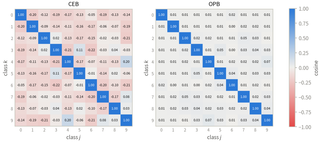
Figure 5: Pairwise-cosine Gram matrix of the posterior class centers on MNIST, averaged over five runs. OPB is nearly diagonal: the posterior centers are orthogonal; CEB shows no such structure.
