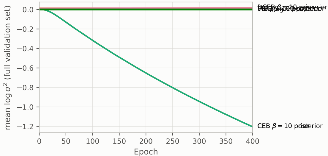
Long-horizon variance trajectories (400 epochs, \beta = 10 , run 1)
