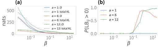
Figure 1: Alignment and separation diagnostics over the ImageNet-100 compression sweep. (a) Anchor mismatch \hat{D} (solid) and total KL (dashed) against \beta , by anchor scale. (b) Fraction of class pairs with a positive separation lower bound.
