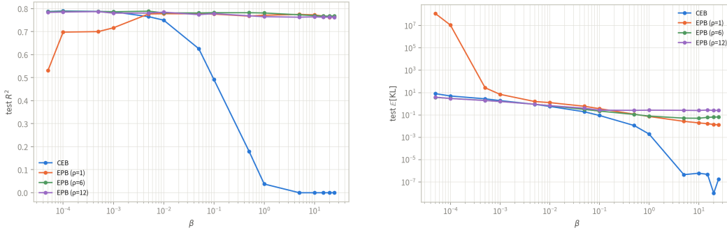
Figure 8: California Housing compression sweep (MLP). Left: test R^2 ; right: realized conditional KL over \beta . EPB maintains a task plateau through strong compression, while the \rho = 1 weak-compression points exhibit a large variance term.
