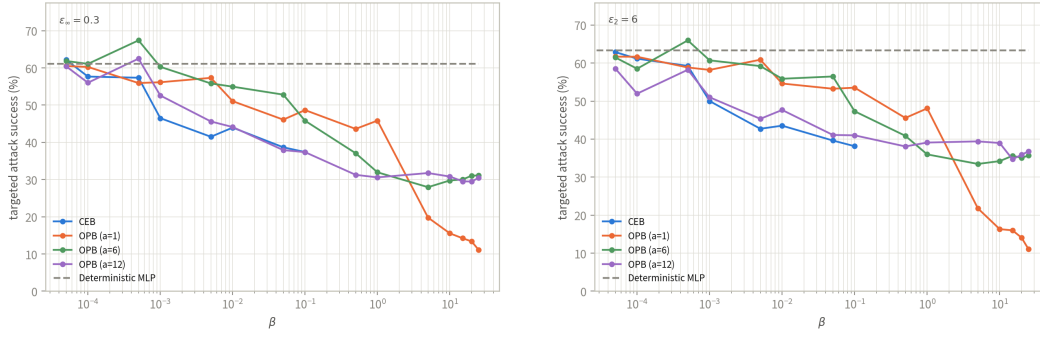
Figure 3: Targeted PGD attack success rate against \beta (log scale) on MNIST (MLP backbone): target class 0, 20 steps, EOT-10 gradients and 10-sample MC predictions on the stochastic path. (a) L_\infty , \varepsilon = 0.3 ; (b) L_2 , \varepsilon = 6.0 . The dashed grey line is the deterministic MLP baseline; CEB is drawn over its operating range only ( \beta \leq 0.1 ), beyond which its reference collapses to chance. Every curve falls with \beta , and OPB keeps gaining robustness across the entire grid: at \beta = 25 , OPB ( a = 1 ) reaches 11% — 50 points below the baseline.
