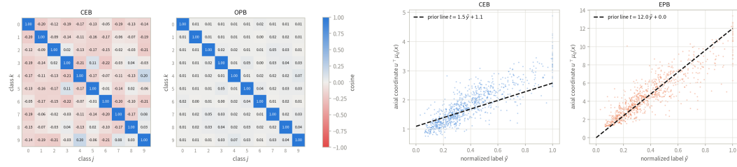
Figure 5: Posterior geometry at the matched operating point: class-center Gram matrix (left) and EPB axial coordinates (right).
