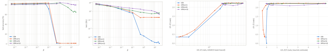
Figure 4: Compression diagnostics across two views and two tasks. (a)–(b) ImageNet-100 classification sweep (MLP): test accuracy and realized conditional KL against \beta ; CEB and the smallest anchor collapse at strong compression, whereas a = 12 retains the plateau. The Housing regression counterpart is provided in Appendix B.3. (c)–(d) MNIST information-plane and certificate-plane estimates (estimator-level diagnostics rather than mutual-information identities; Appendix B.4).
