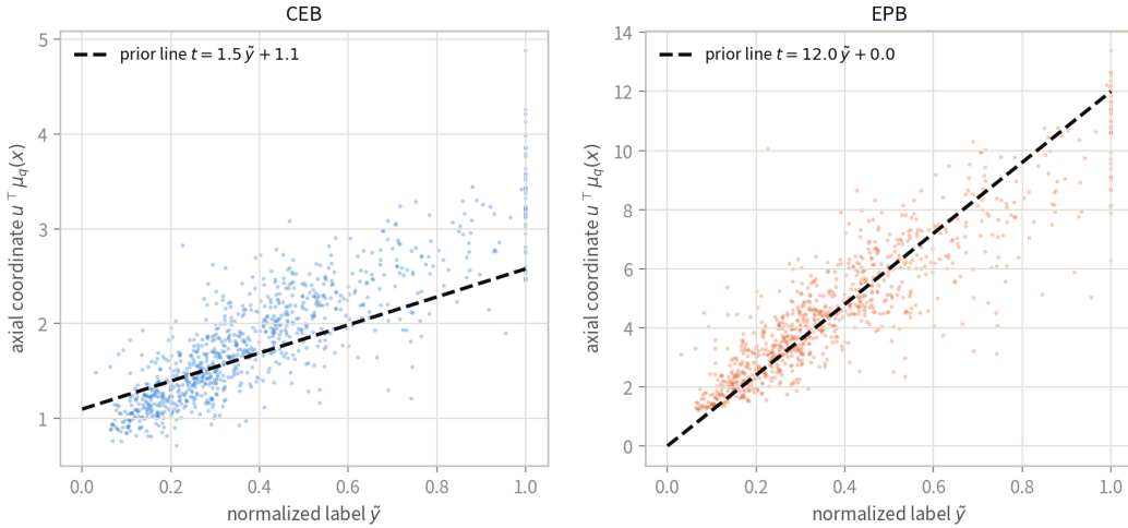
Figure 3: The axial coordinate u^\top \mu_q(x) against the normalized label on Housing (one representative run per model). The EPB posterior hugs the prior line \rho \tilde{y} , shrunk toward \rho \mathbb{E}[\tilde{y} | x] by the encoder’s uncertainty.
