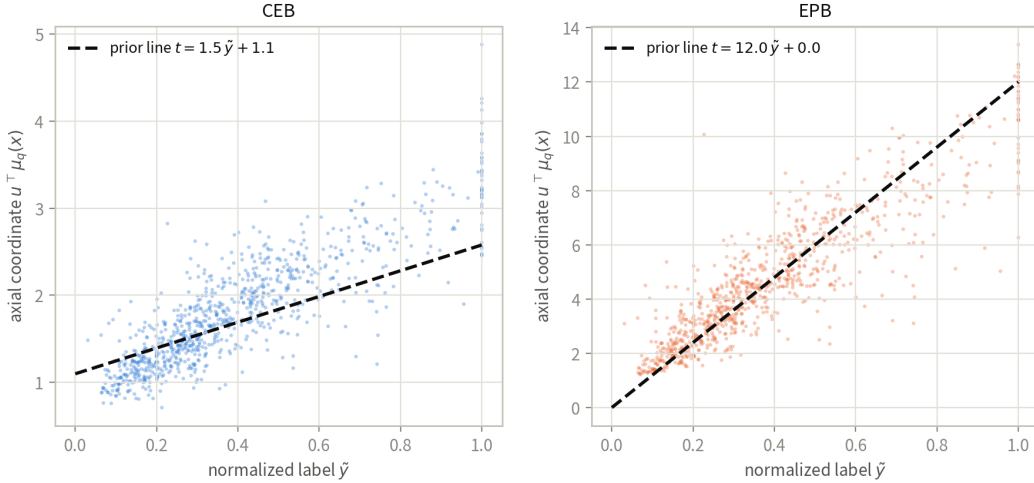
Figure 5: The axial coordinate u^\top \mu_q(x) against the normalized label on Housing (one representative run per model). The EPB posterior hugs the prior line \rho \tilde{y} , shrunk toward \rho \mathbb{E}[\tilde{y} | x] by the encoder’s uncertainty.
