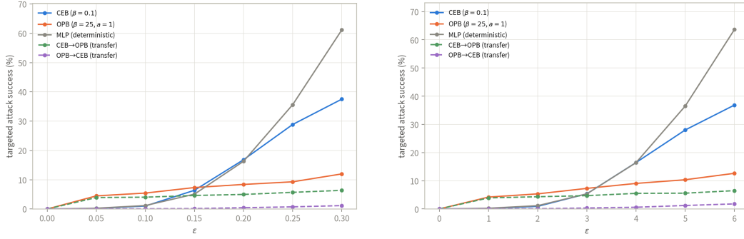
Figure 3: Transfer attacks (gradient-masking check) on MNIST (MLP backbone): targeted PGD adversaries generated on one model and evaluated on another, against \epsilon . (a) L_\infty ; (b) L_2 . Solid: white-box self-attacks of CEB ( \beta = 0.1 ), OPB ( \beta = 25 , a = 1 ) and the deterministic MLP baseline. Dashed: transfer attacks. CEB→OPB stays at or below OPB’s own white-box attack, so OPB’s extreme-compression robustness is not gradient masking; OPB→CEB transfers almost nothing, as the collapsed posterior’s perturbations carry little transferable signal.
