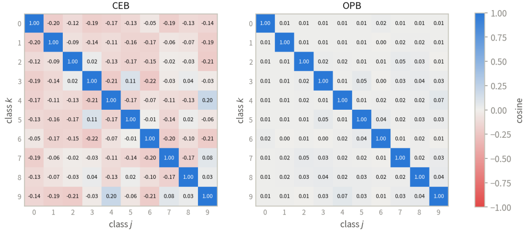
Figure 4: Pairwise-cosine Gram matrix of the posterior class centers on MNIST, averaged over five runs. OPB is nearly diagonal: the posterior centers are orthogonal; CEB shows no such structure.
