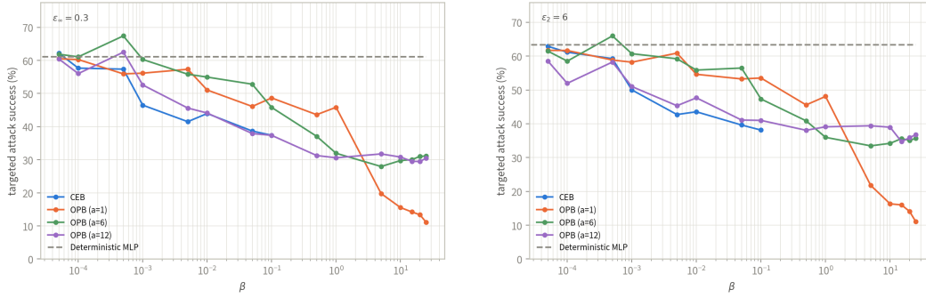
Figure 2: Targeted PGD attack success rate against \beta (log scale) on MNIST (MLP backbone): target class 0, 20 steps, EOT-10 gradients and 10-sample MC predictions on the stochastic path. (a) L_\infty , \varepsilon = 0.3 ; (b) L_2 , \varepsilon = 6.0 . The dashed grey line is the deterministic MLP baseline; CEB is drawn over its operating range only ( \beta \leq 0.1 ), beyond which its reference collapses to chance. Every curve falls with \beta , and OPB keeps gaining robustness across the entire grid: at \beta = 25 , OPB ( a = 1 ) reaches 11% — 50 points below the baseline.
