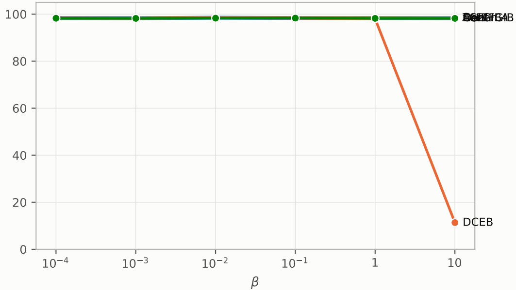
(b) Confound ablations on MNIST/MLP ( a = 16 )
