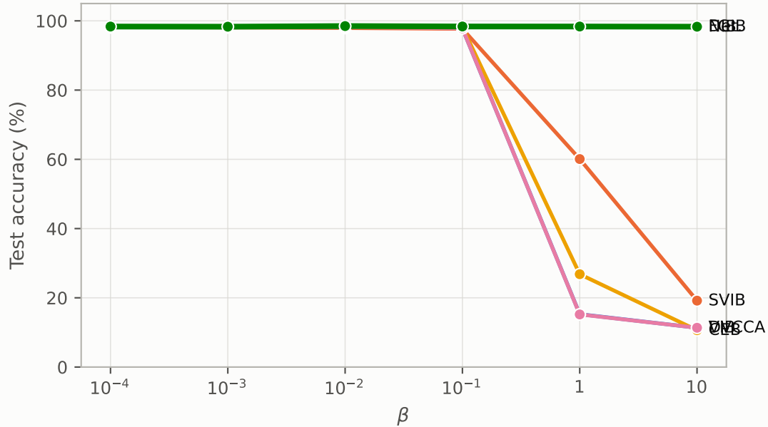
(a) Objectives on MNIST/MLP
