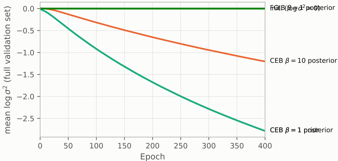
Long-horizon variance trajectories (400 epochs, run 1)
