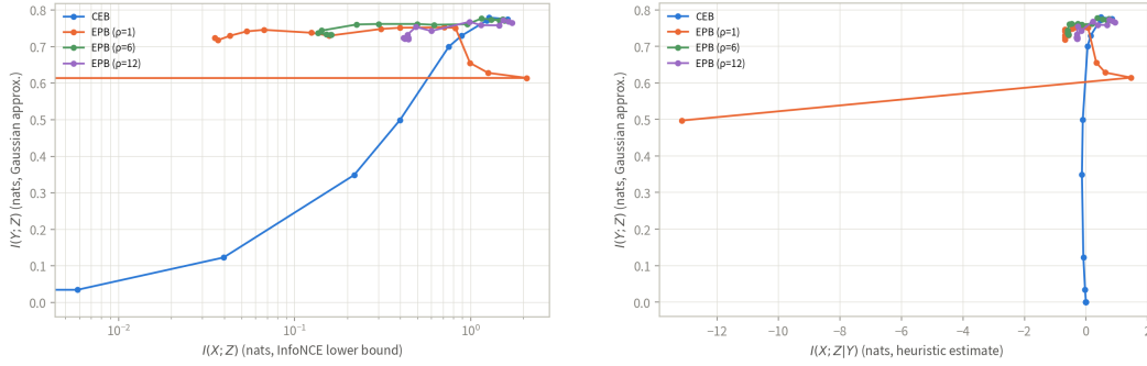
Figure 7: Information plane (a) and certificate plane (b) for Cal. Housing, companion panels to Fig. 2(c,d): identical estimators, \beta grid (log x -scale in (a); linear where the estimated residual turns negative in (b)), five runs per point, lines connect \beta in ascending order. CEB one curve per panel; EPB three ( \rho \in \{1, 6, 12\} ).
