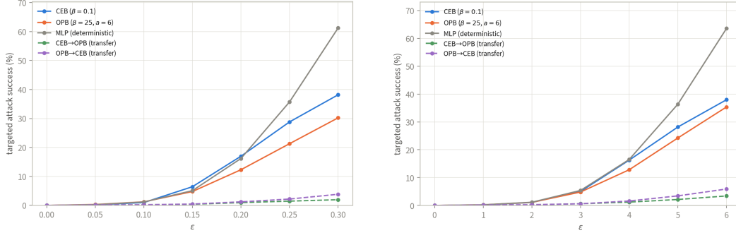
Figure 9: Transfer PGD curves on MNIST (gradient-masking check). Targeted adversaries are generated on one model and evaluated on another; CEB-to-OPB transfer remains far below OPB’s own white-box attack. The targeted white-box curves are in the main text.
