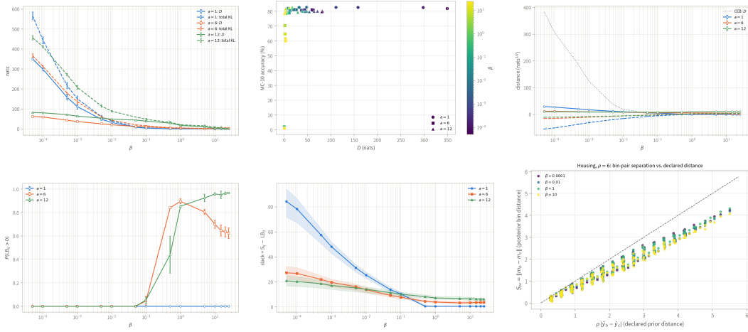
Figure 1: Direct mismatch diagnostics over the compression sweeps. (a) ImageNet-100 anchor mismatch \hat{D} and total KL against \beta , by anchor scale. (b) MC-10 accuracy against \hat{D} ; color denotes \beta and marker shape the anchor scale. (c) Mean posterior-center distance (solid) and the raw, unclipped mismatch-dependent lower bound (dashed) against \beta ; the gray dotted line is CEB’s mismatch, shown only as a descriptive reference. (d) Fraction of class pairs with a positive lower bound. (e) The 5th, 50th, and 95th percentiles of the separation slack. (f) Cal. Housing bin-pair separation S_{bc} against the declared prior distance \rho|\bar{y}_b - \bar{y}_c| at \rho = 6 , colored by \beta ; the identity line denotes exact scale transfer. Means and standard deviations are over five seeds; no checkpoint is omitted. The remaining Housing panels are in Appendix A.6.
