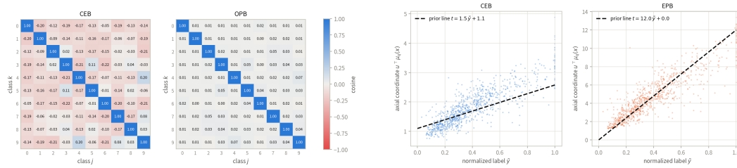
Figure 4: Posterior geometry at the matched operating point: class-center Gram matrix (left) and EPB axial coordinates (right).
