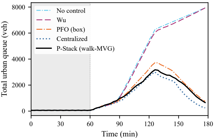
Urban queue trajectory — High demand
