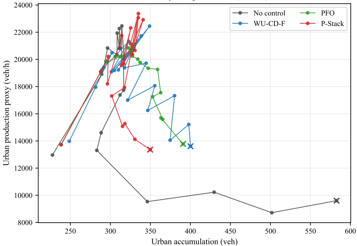
Urban MFD Operating-Point Shift (Incident)
