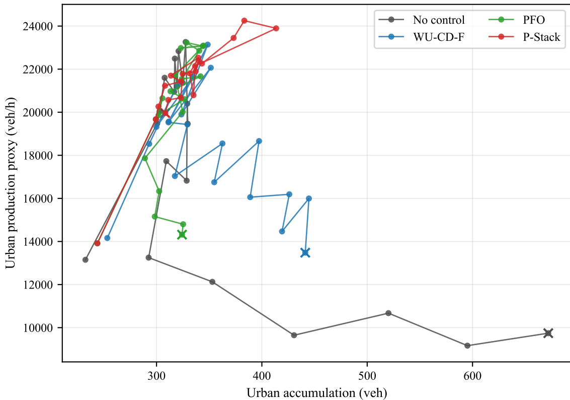
Urban MFD Operating-Point Shift (Peak)
