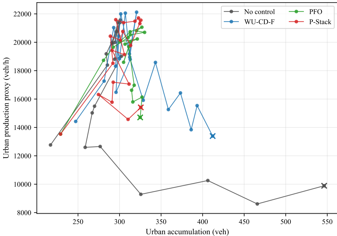
Urban MFD Operating-Point Shift (Peak skew)
