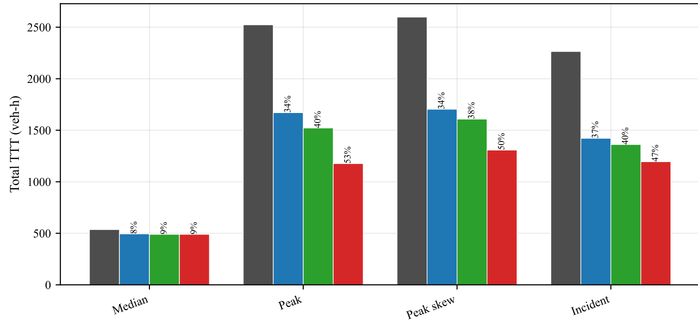
Fig. 1A. Total TTT Across Focus Scenarios
