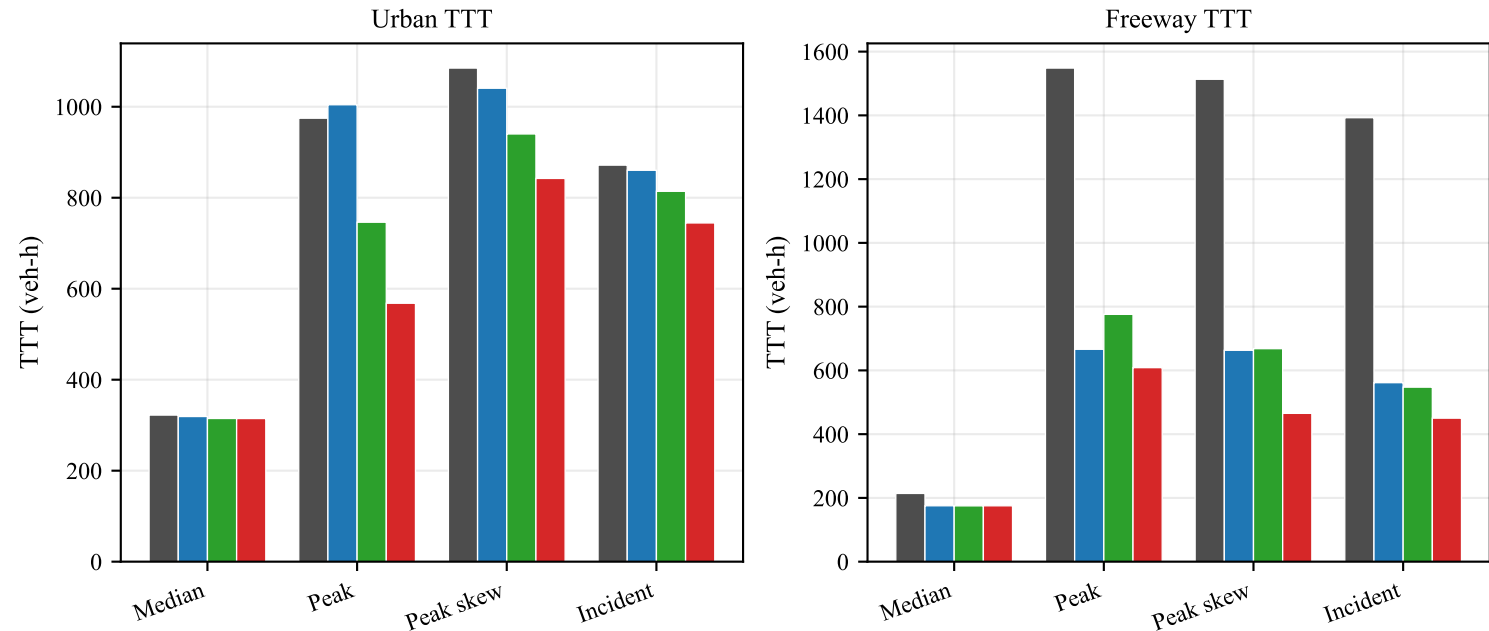
Fig. 1B. Urban-Freeway TTT Burden Decomposition
