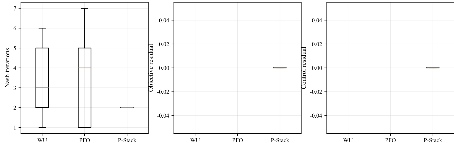
Fig. 4A. Follower Nash/Response Diagnostics
