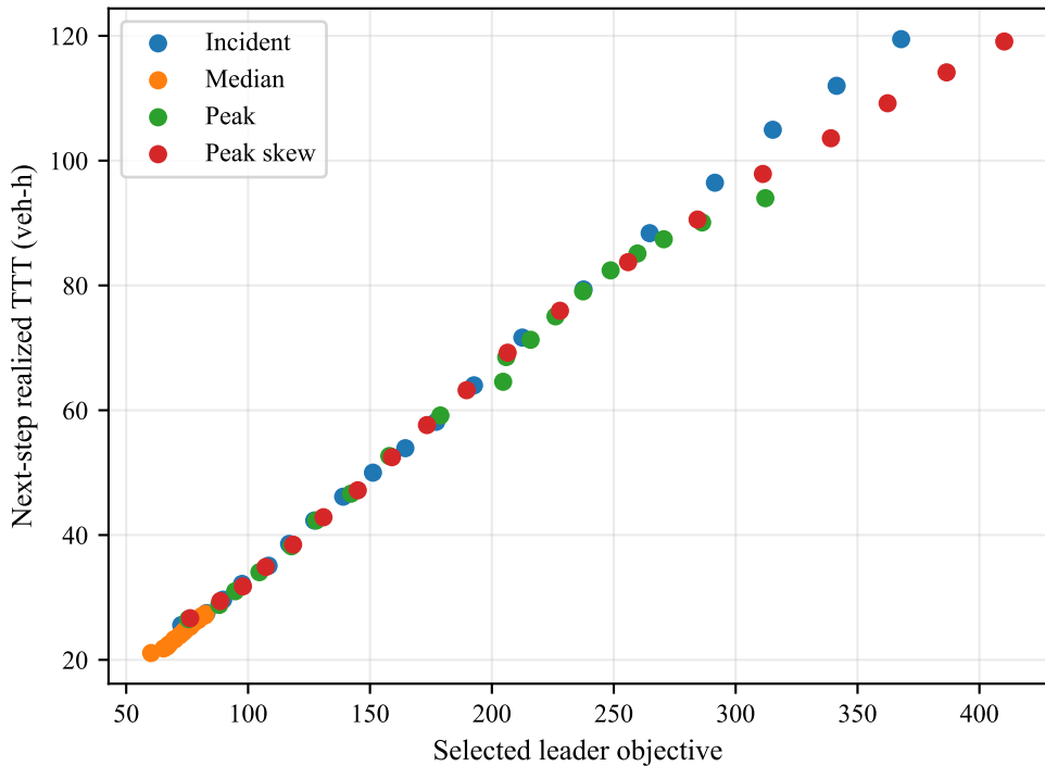
Fig. 4D. Selected Objective vs Realized Plant TTT
