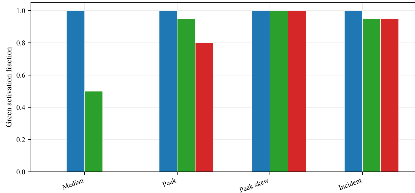
Fig5C green activation
