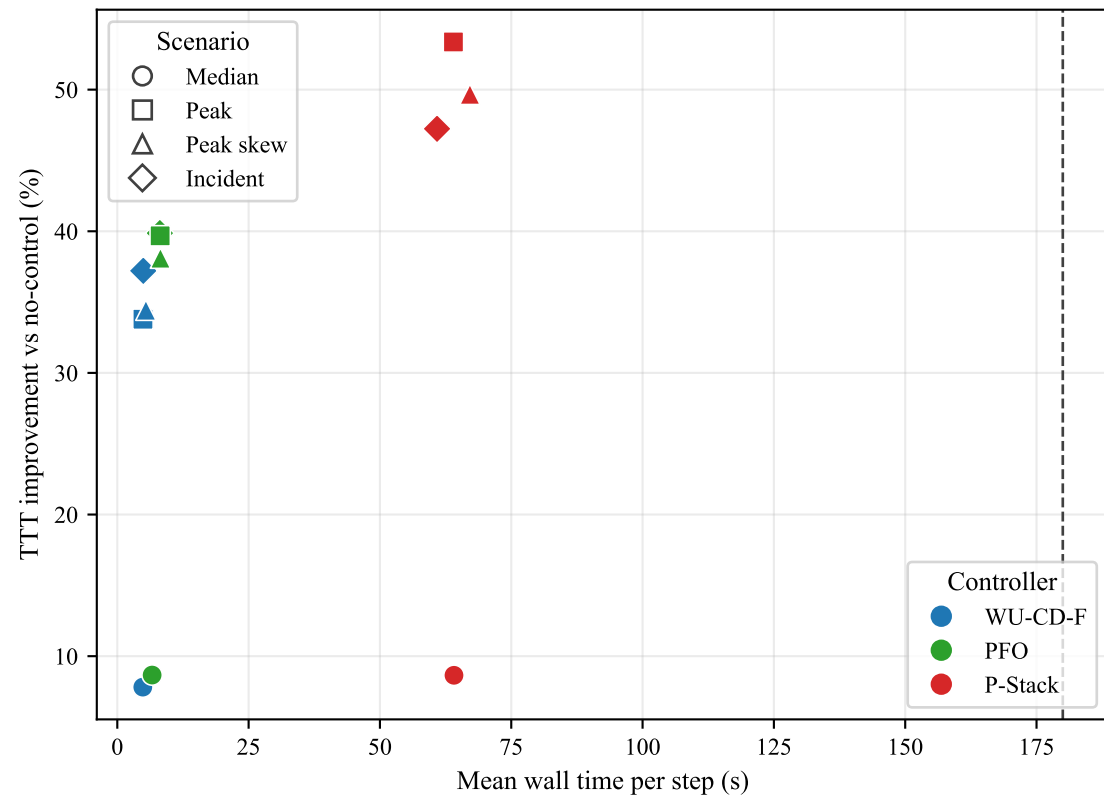
Fig. 6C. Performance-Compute Trade-Off
