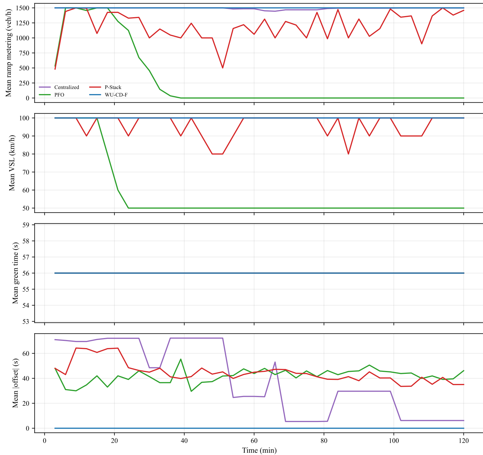
Incident Micro-Control Behavior
