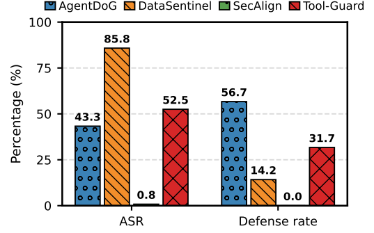
Figure 6: ECLIPSE under potential defense mechanisms. Bars report ASR and defense rate for each mechanism; SecAlign’s zero defense rate is a result of its model-level refusal interface.
