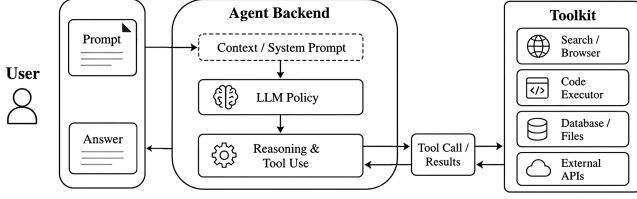
Figure 1: The workflow of LLM agent system.
