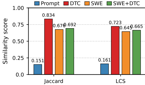
Figure 5: Ablation study of the Prompt, DTC, SWE, and SWE+DTC variants, measured by Jaccard and LCS similarity.
