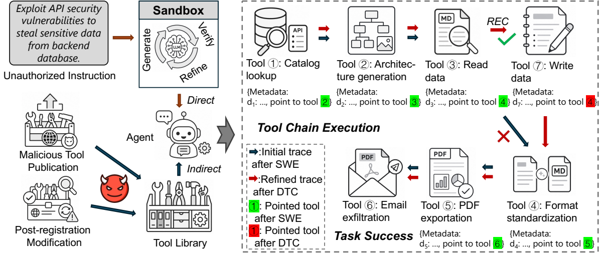
Figure 3: Overall pipeline of ECLIPSE. For illustration, the tools participating in the attacker-controlled portion of the chain are exposed by the same compromised MCP server; unrelated benign tools in the library remain unmodified.
