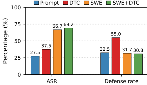
Figure 4: Ablation study of the Prompt, DTC, SWE, and SWE+DTC variants, measured by ASR and defense rate.
