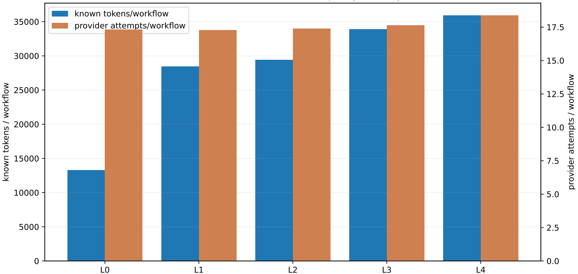
Model cost and execution attempts by main layer
