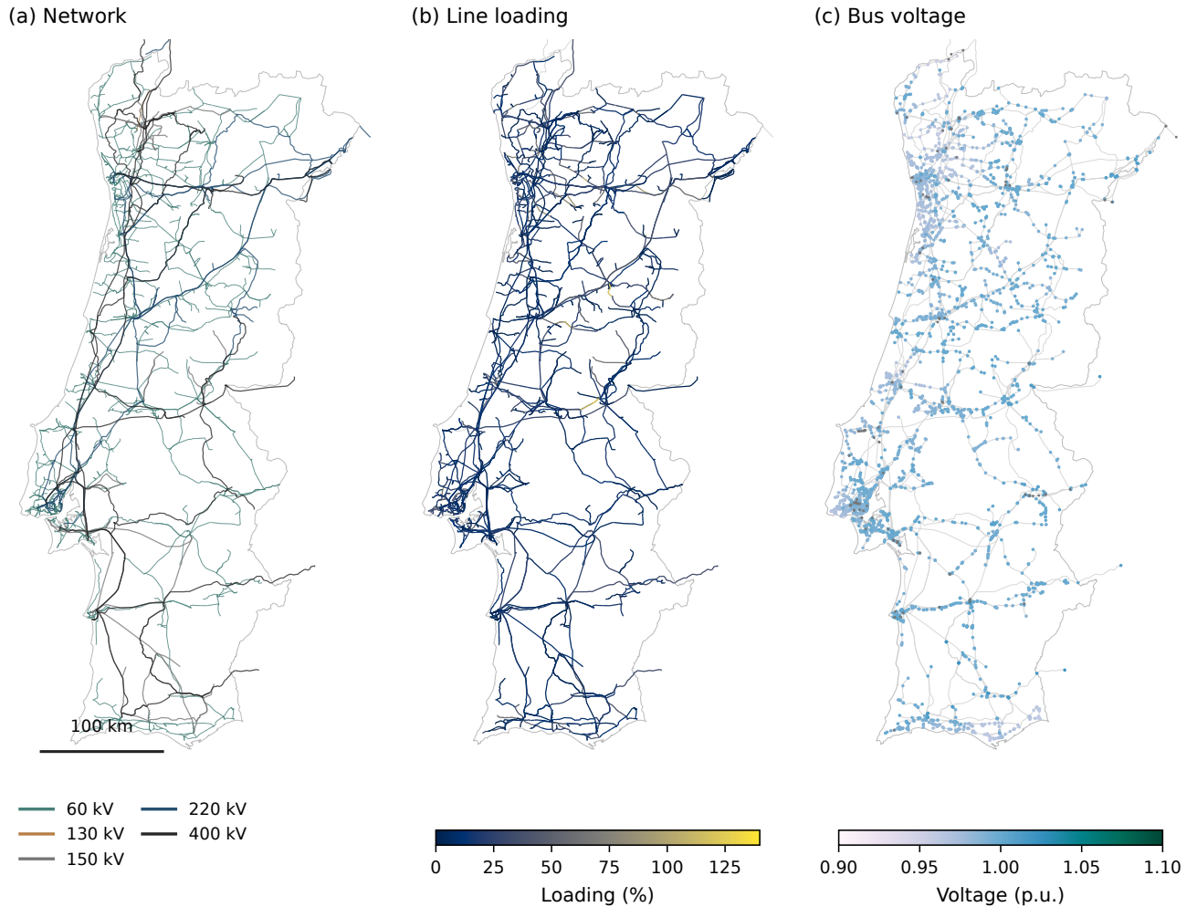
Figure 1—Geographic network and solved state at the annual peak. (a) The 60–400 kV network containing
