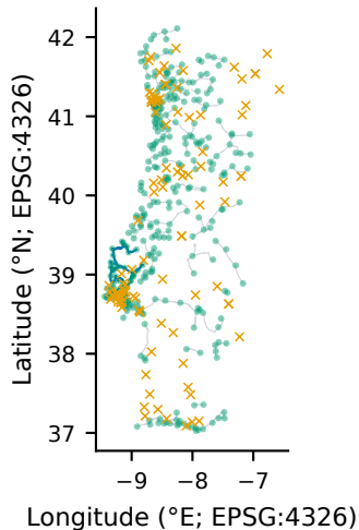
a Released candidate geography
