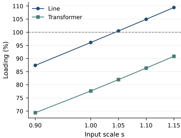
(a) Maximum loading
