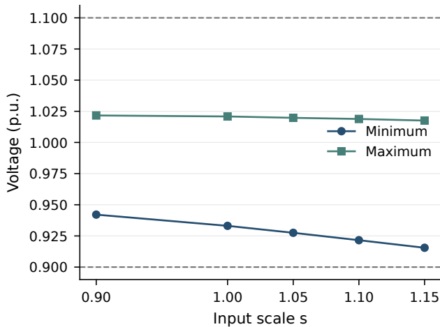
(b) Voltage extrema
