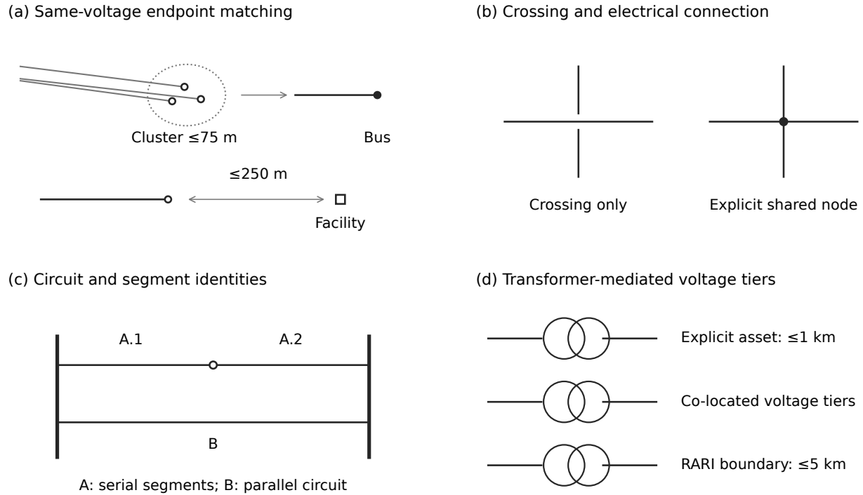
Figure 1—Connection rules used in static-network reconstruction. (a) Same-voltage endpoint clustering and facility matching; (b) distinction between geometric crossings and explicit shared nodes; (c) preservation of series segments and parallel-circuit identity; and (d) cross-voltage connection from explicit equipment, colocated facilities, and RARI boundary evidence. The diagrams are abstract electrical schematics rather than geographic device locations. Distance thresholds and fallback rules are listed in Table 3.
