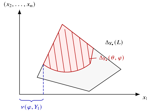
Fig. 10.1 The first-coordinate support of the partial Okounkov body.
