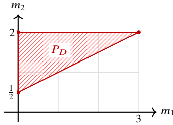
Fig. 12.5 A surface example where P_D is not a lattice polytope.
