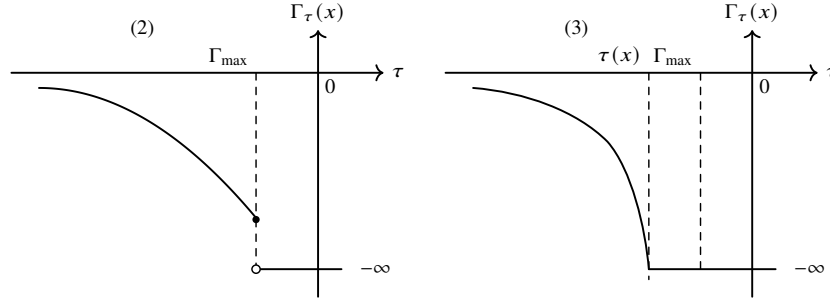
Fig. 9.1 The last two pointwise possibilities for \tau \mapsto \Gamma_\tau(x) .
