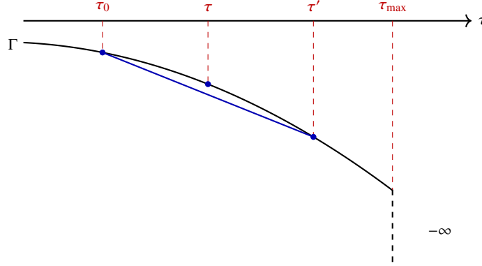
Fig. 9.2 The test curve \Gamma .
