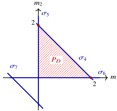
Fig. 12.4 The polytope P_D for D = 2D_{\sigma_4} + D_{\sigma_7} . The blue lines are the four affine hyperplanes a_\rho + \langle m, u_\rho \rangle = 0 for \rho \in \Sigma(1) .
