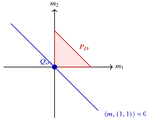
Fig. 12.7 The face Q_{\sigma_7} = \{m \in P_D : \langle m, (1, 1) \rangle = 0\} is the single point \{(0, 0)\} , of dimension 0 rather than the expected 1.
