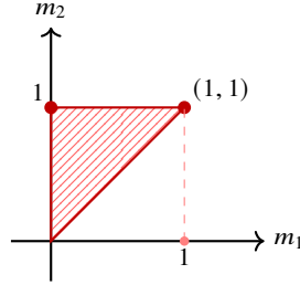
Fig. 12.6 The Okounkov body \Delta_{Y_*}(\mathrm{Bl}_0\mathbb{P}^2, \pi^* \mathcal{O}_{\mathbb{P}^2}(1)) .
