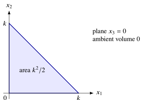
Fig. 20.1 For the Hopf threefold and k > 0 , the body is a triangle in a coordinate plane. Its area gives the quadratic section growth, while its ambient volume vanishes.
