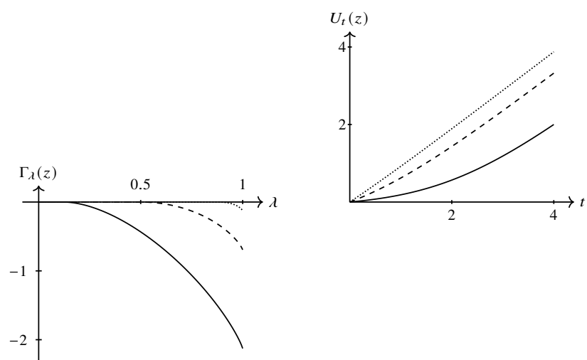
Fig. 18.1 The explicit test curve and its ray, at points with \log |z|^2 = -2 (solid), 0 (dashed), and 2 (dotted). The parameter functions on the left are concave; their transforms on the right are convex.
