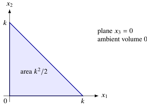
Fig. 21.1 For the Hopf threefold and k > 0 , the body is a triangle in a coordinate plane. Its area gives the quadratic section growth, while its ambient volume vanishes.
