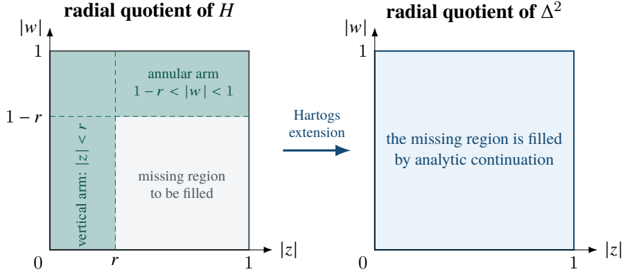
Figure 2.1: The map q : \Delta^2 \rightarrow [0, 1]^2 , q(z, w) = (|z|, |w|) , collapses the S^1 \times S^1 orbits. In this radial quotient the Hartogs figure is the shaded L-shaped set on the left. Its envelope of holomorphy is the full bidisc, represented by the filled square on the right. Thus this is a quotient picture of a four-real-dimensional domain, not a literal planar cross-section.
