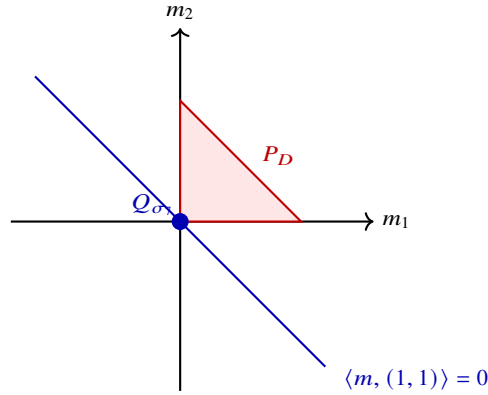
Fig. 12.5 The face Q_{\sigma_j} = \{m \in P_D : \langle m, (1, 1) \rangle = 0\} is the single point \{(0, 0)\} , of dimension 0 rather than the expected 1.
