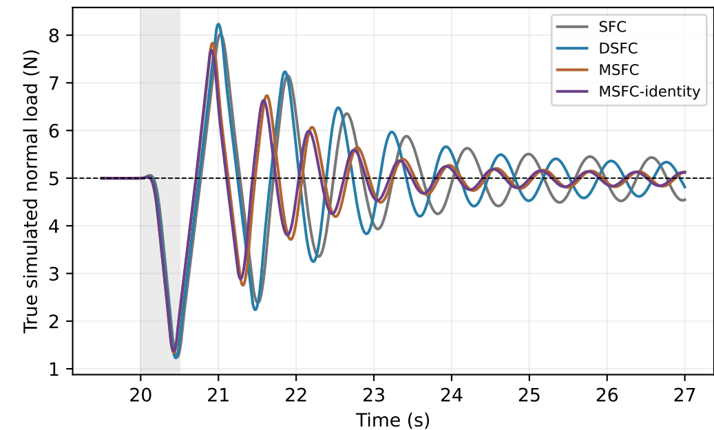
FP-v1: fixed 3 N, 0.5 s oblique pulse with frozen normal observer Development simulation; untuned candidates. Identity metric retains force-history states.
