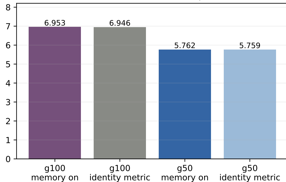
Nominal path RMS (mm)
