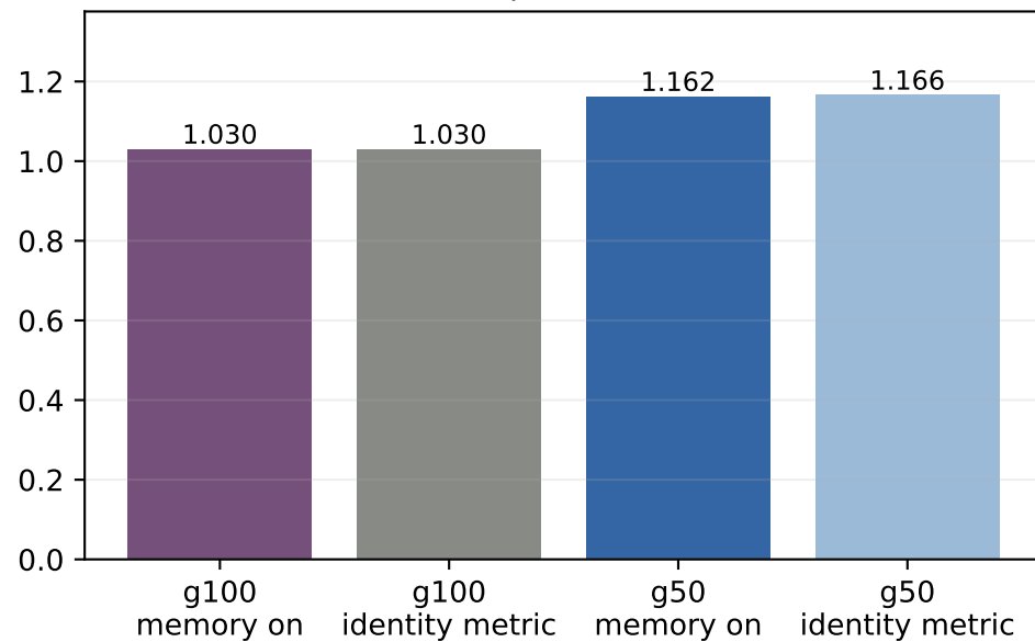
Nominal path RMS (mm)
