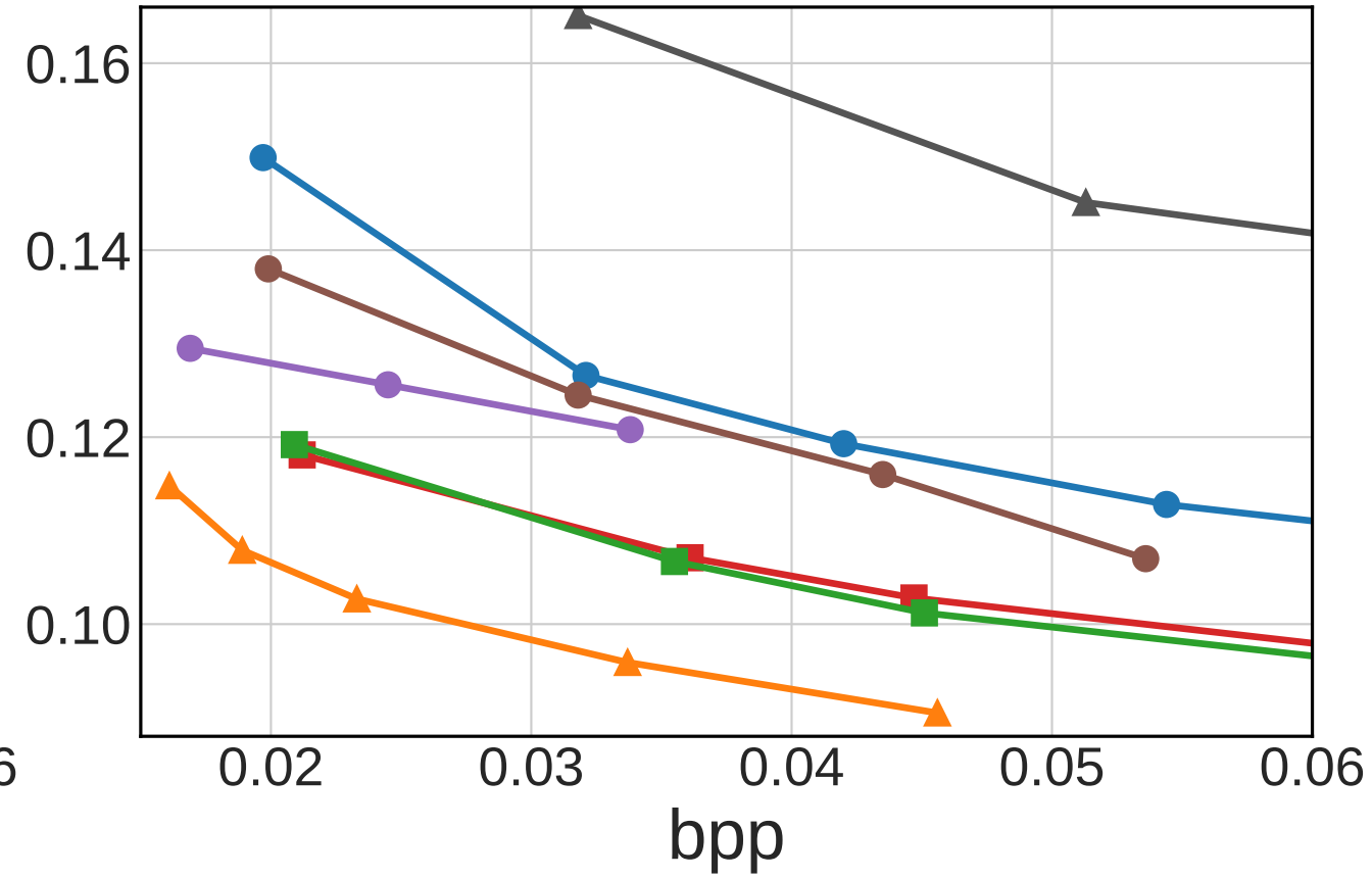
DISTS ↓
