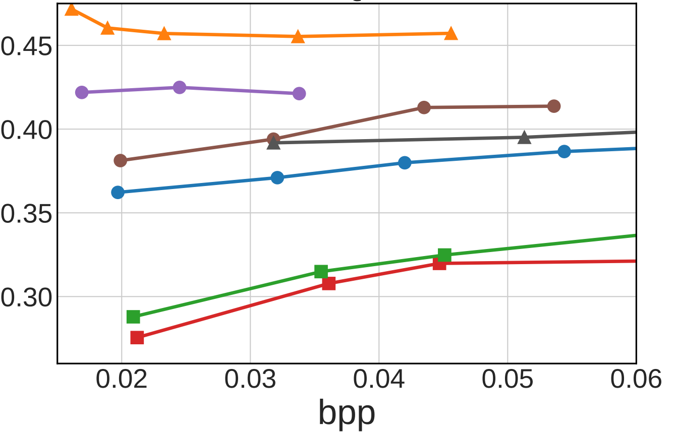
CLIQQA ↑
