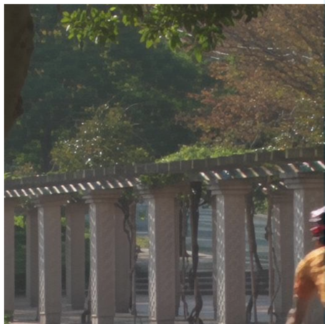
Diff-SIT (0.0259)
