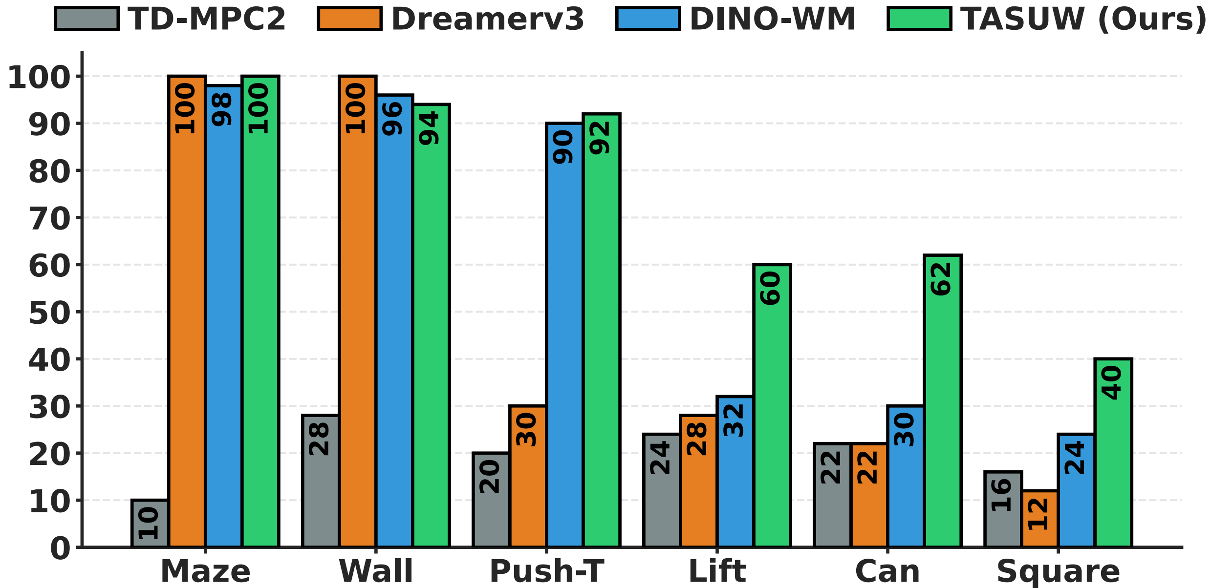
Success Rate (%)
