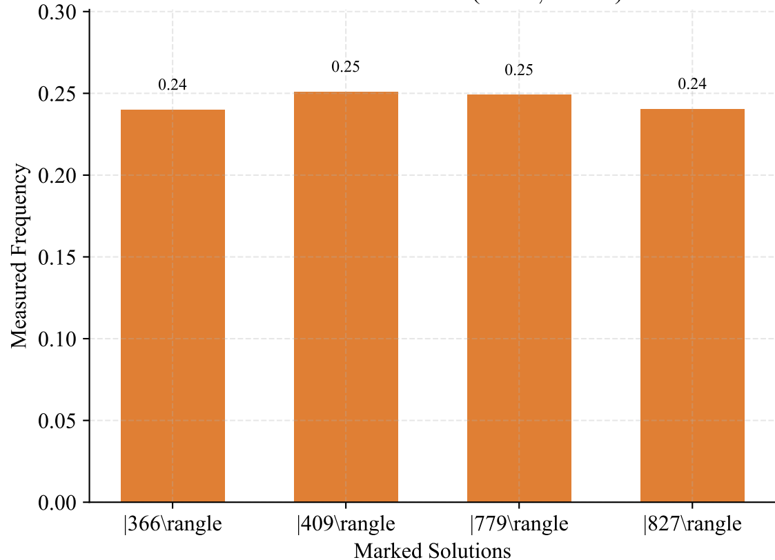
Solution Distribution ( k = 4, t = 13 )
