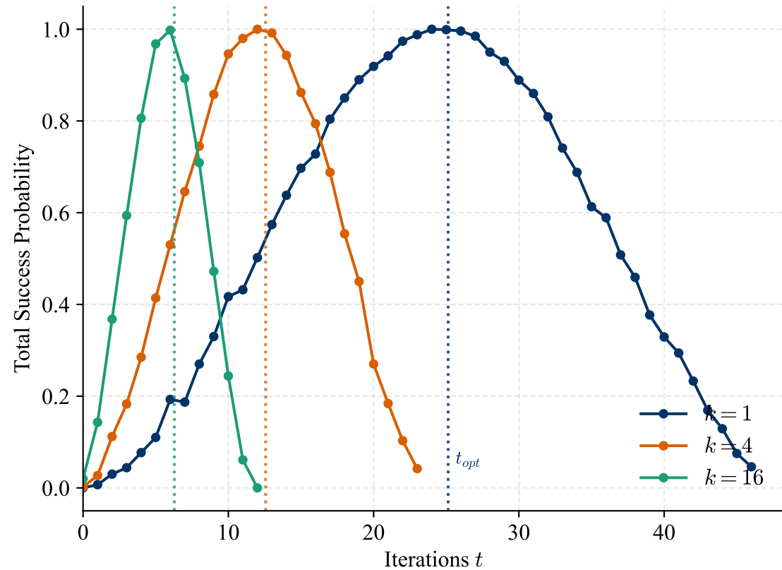
Convergence Speedup ( N = 2^{10} )
