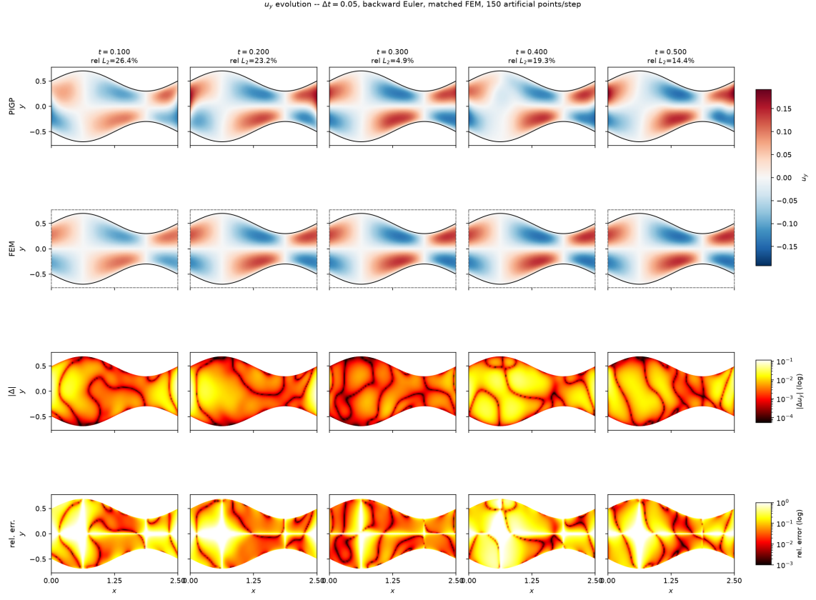
Figure 8: Evolution of u_y , 150 artificial points per step.
