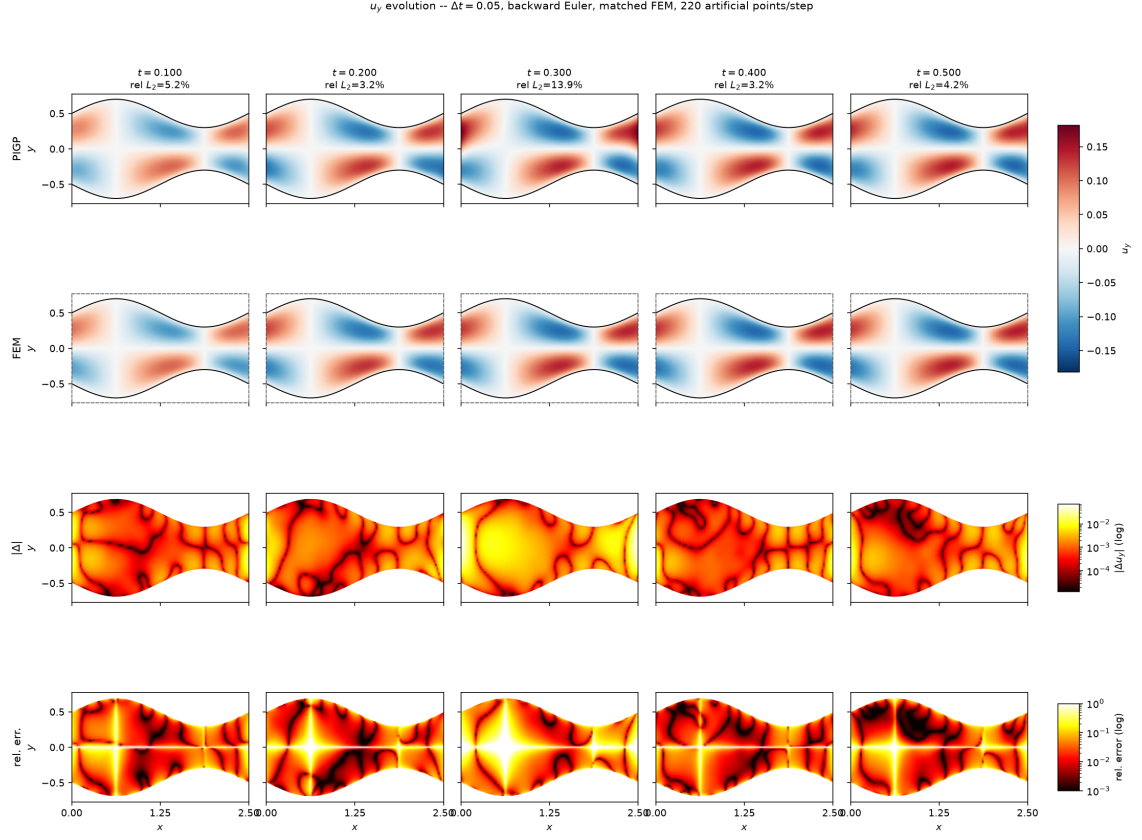
Figure 10: Evolution of u_y , 220 artificial points per step.
