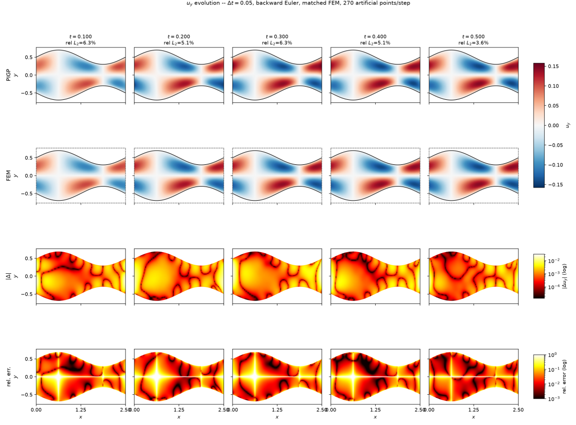
Figure 12: Evolution of u_y , 270 artificial points per step.
