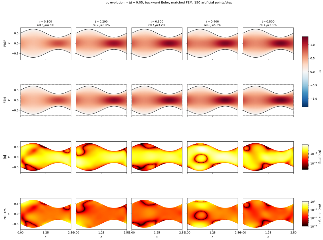
Figure 7: Evolution of u_x , 150 artificial points per step.
