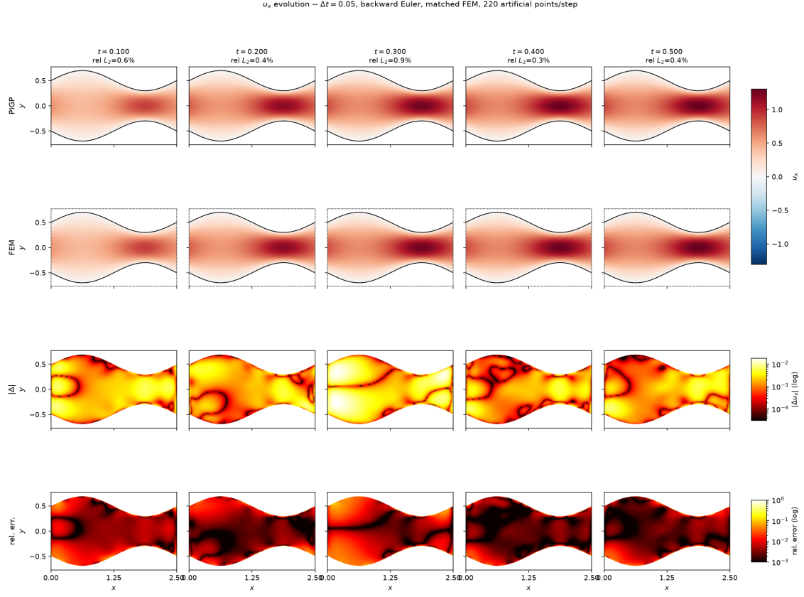
Figure 9: Evolution of u_x , 220 artificial points per step.
