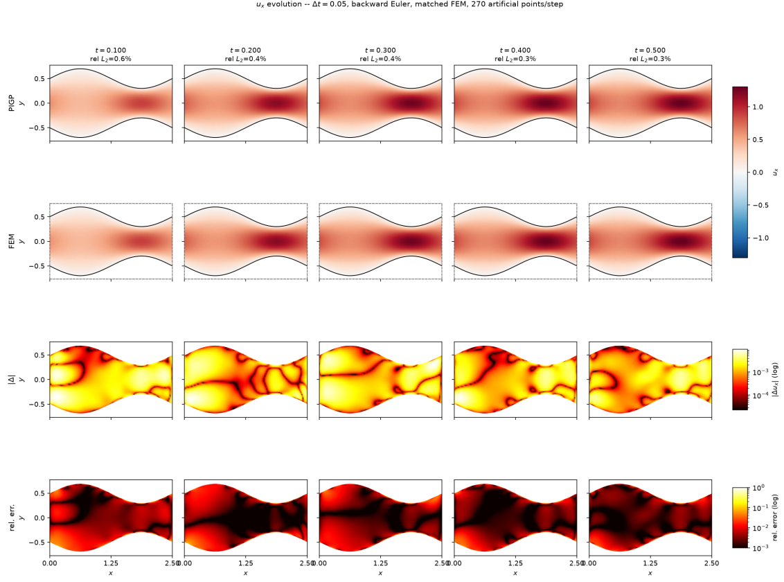
Figure 11: Evolution of u_x , 270 artificial points per step.
