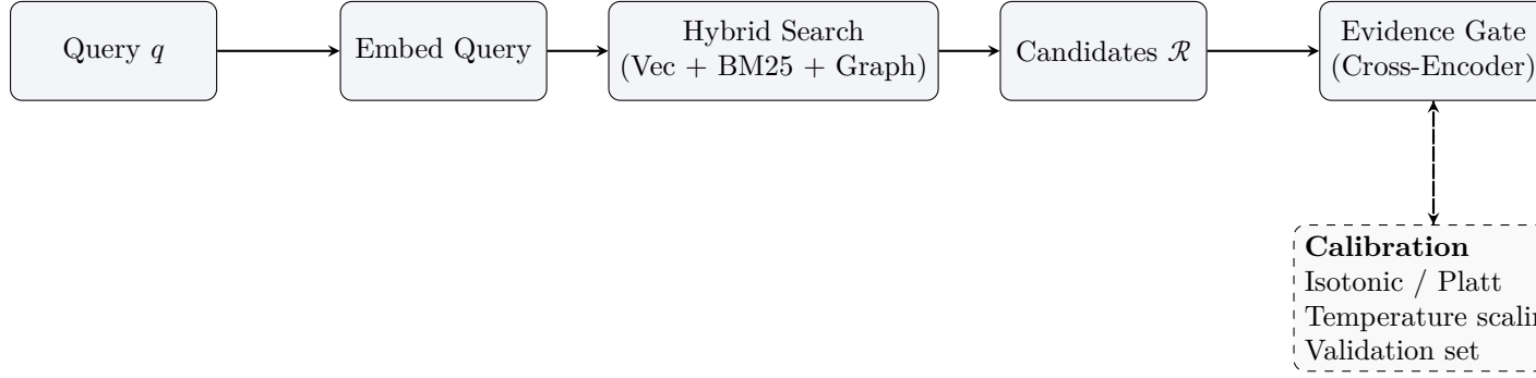
Figure 4.1: Retrieval + Evidence Gate pipeline.
