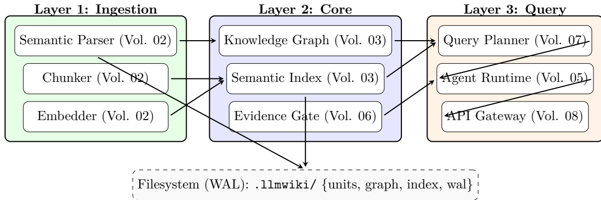
Figure 1.1: Three-Layer Architecture of LLMWiki. Filesystem acts as write-ahead log (WAL) for all layers.
