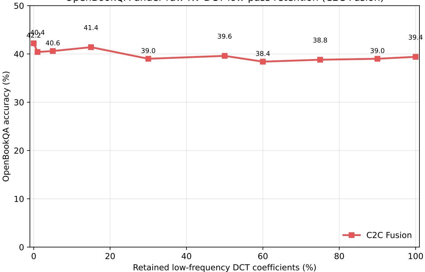
OpenBookQA under raw-KV DCT low-pass retention (C2C Fusion)
