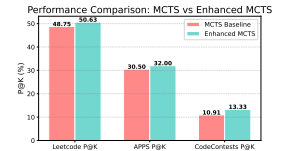
Figure 12: P@K on three benchmarks using the same backbone (GPT-4o-mini), 16 MCTS iterations, and a 6-case self-generated validation set. Injecting our process-oriented layer (strategy pool + momentum)
